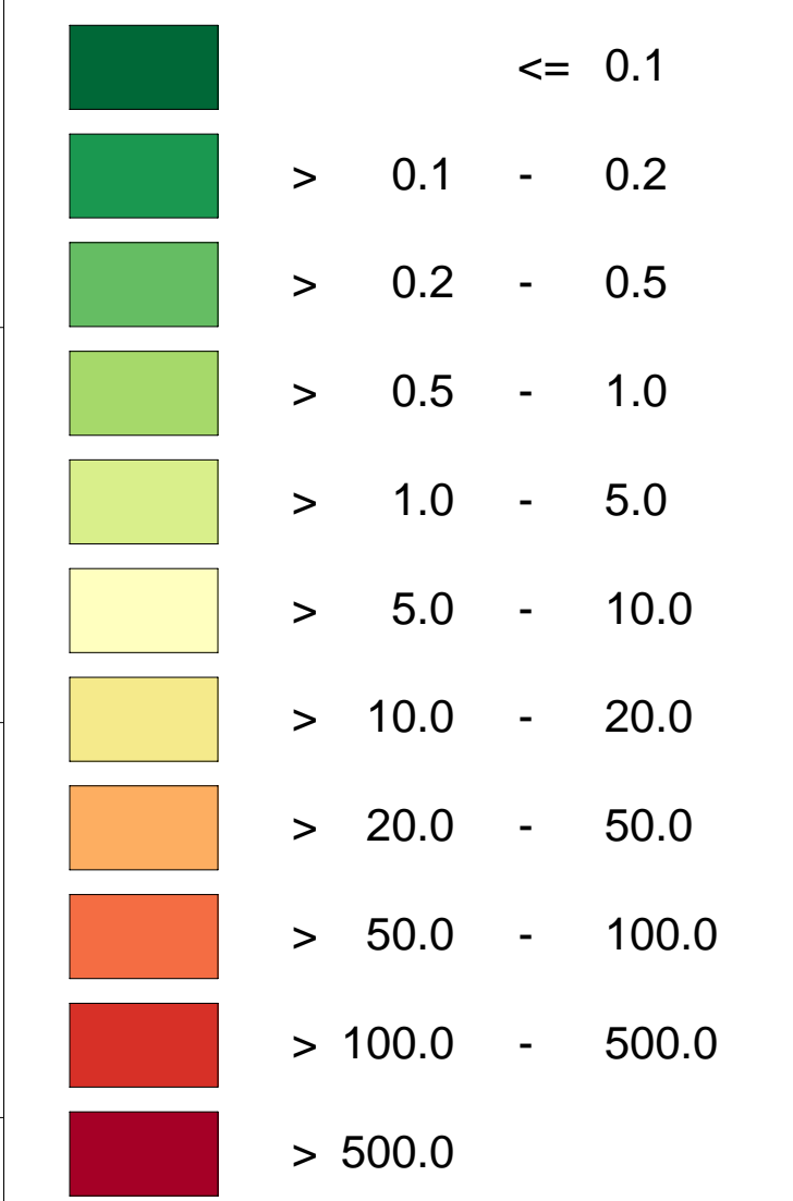
Emissions of Industry 2005 (t/km 2 a)
