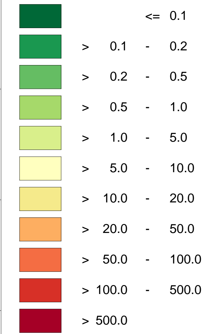
Emissions of domestic fuel 1994 (t/km² a)
