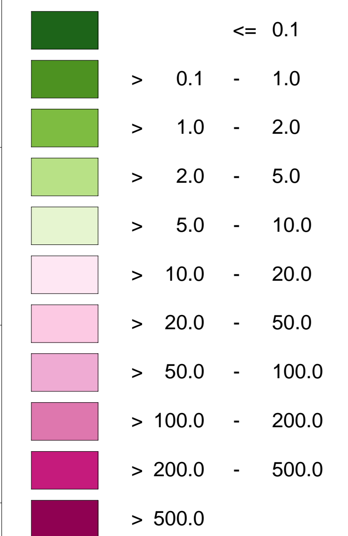
Emissions of all Polluter-Groups 2005 (t/km² a)
